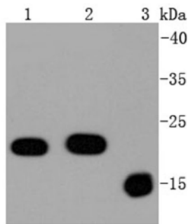
Fig. 1. Western blot analysis of Bax on different lysates using anti-Bax antibody at 1/1,000 dilution. Positive control: Lane 1: Hela; Lane 2: MCF-7; Lane 3: Human liver
